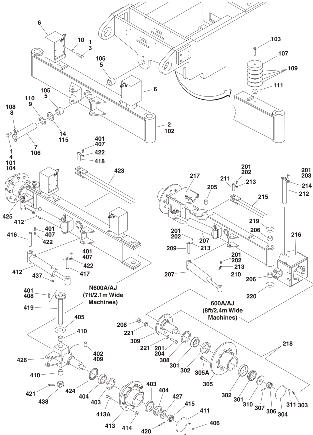
FIGURE 1-1. 2WD FRONT AXLE & STEERING INSTALLATIONS
