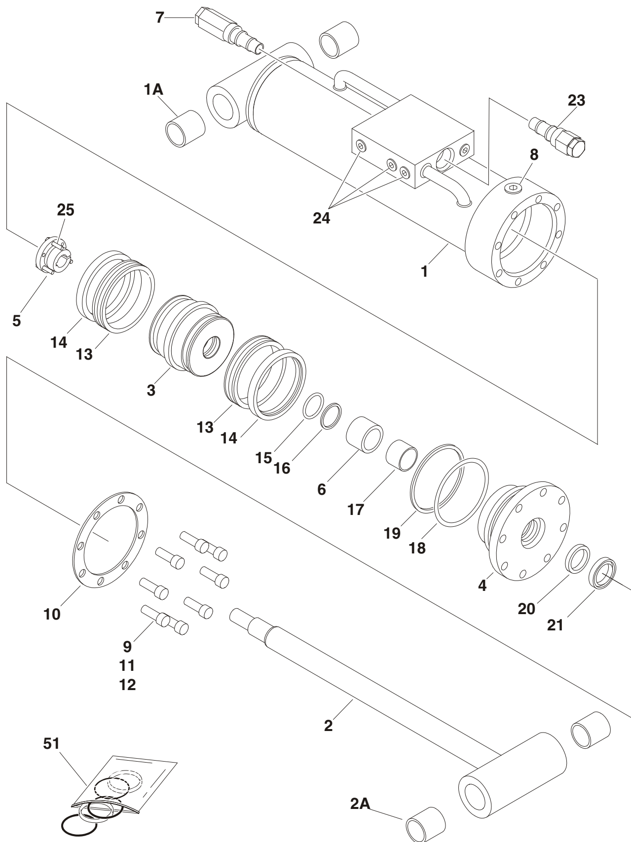
FIGURE 5-2. LEVEL CYLINDER ASSEMBLY - PLATFORM
