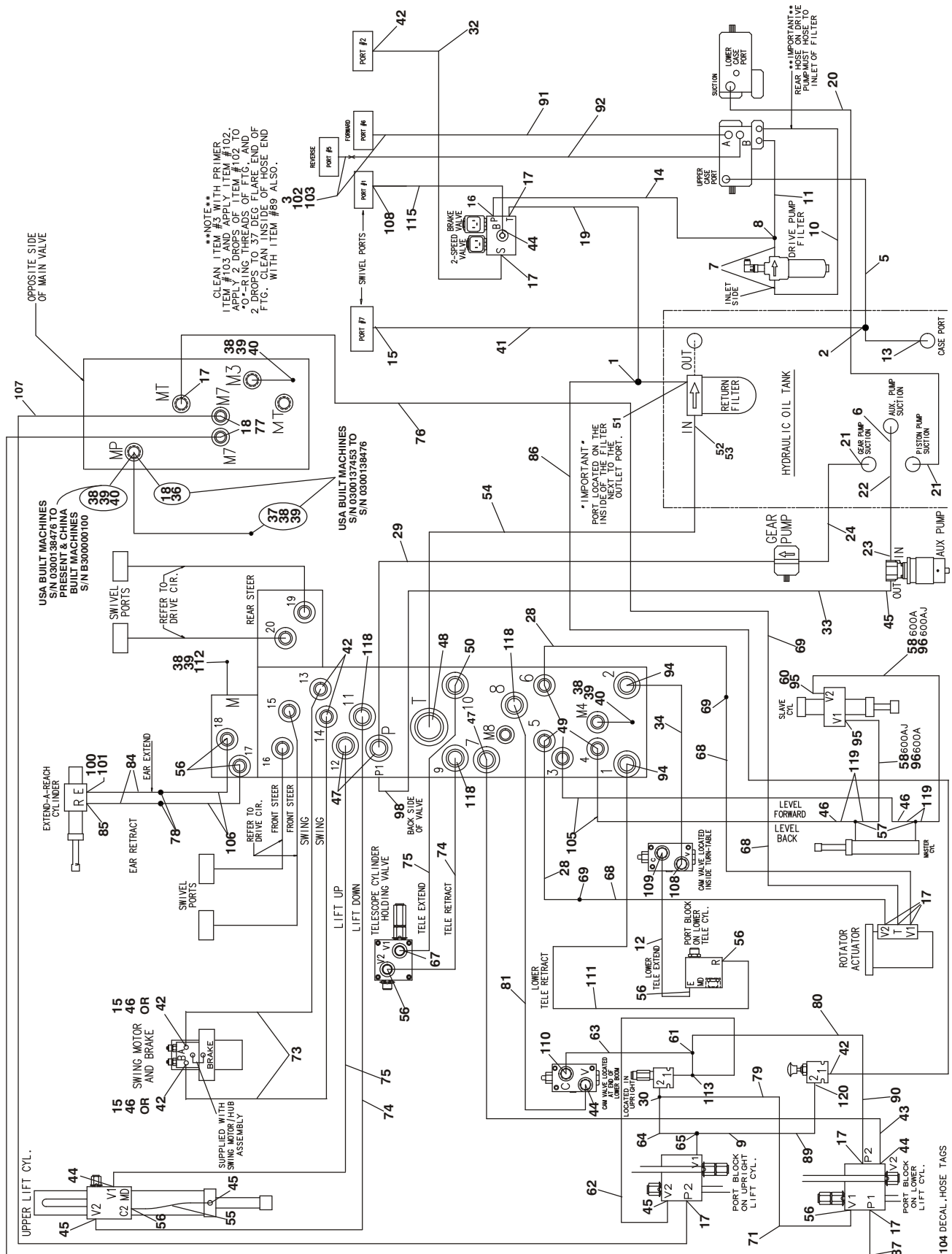
FIGURE 6-5. HYDRAULIC DIAGRAM - STANDARD (USA BUILT MACHINES S/N 0300137453 TO S/N 0300177361 & CHINA BUILT MACHINES S/N B300000100 TO PRESENT)
