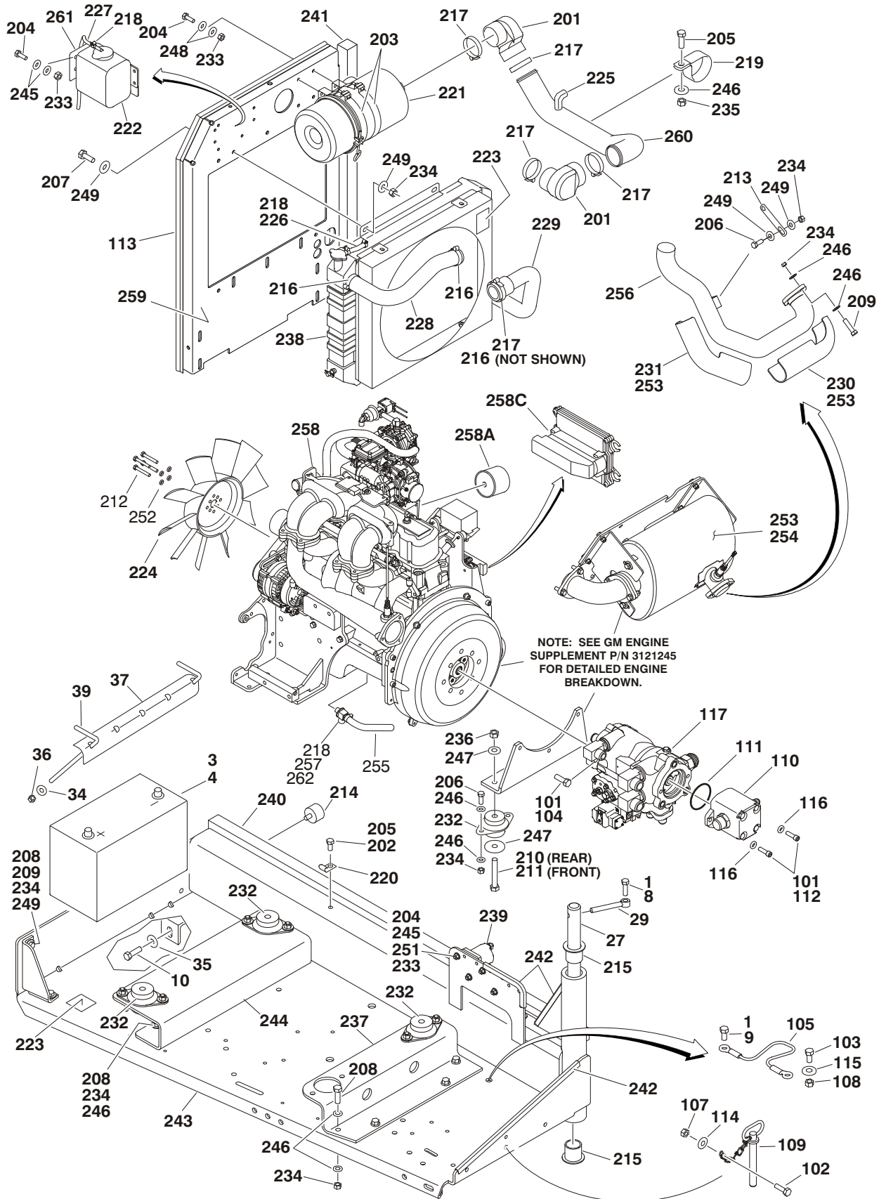
FIGURE 2-14. GM ENGINE INSTALLATION (USA BUILT MACHS S/N 0300139354 TO S/N 0300177361)
