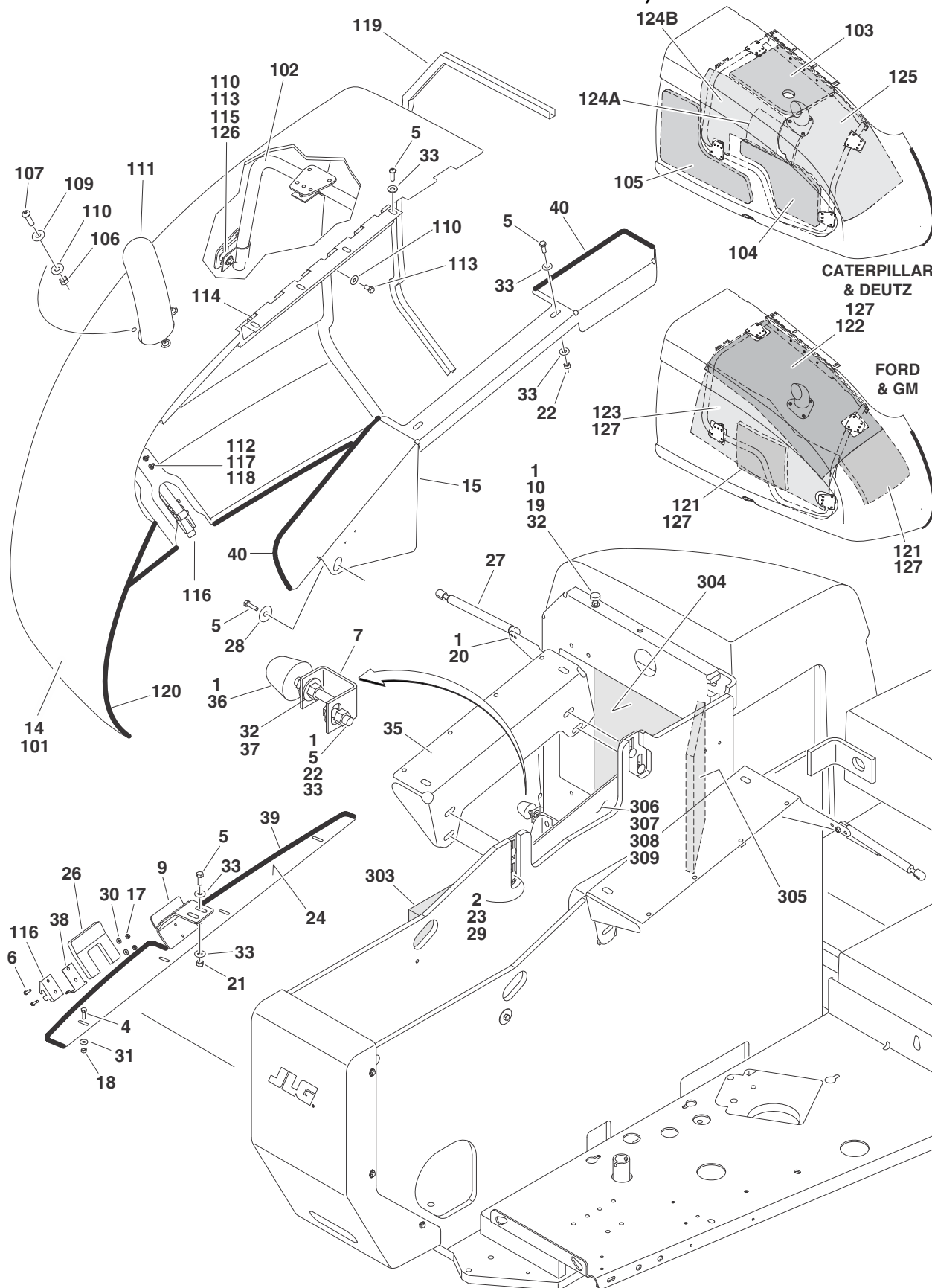
FIGURE 2-25. HOODS INSTALLATIONS (USA BUILT MACHINES S/N 0300089989 TO S/N 0300177361 & CHINA S/N B300000100 TO PRESENT)
