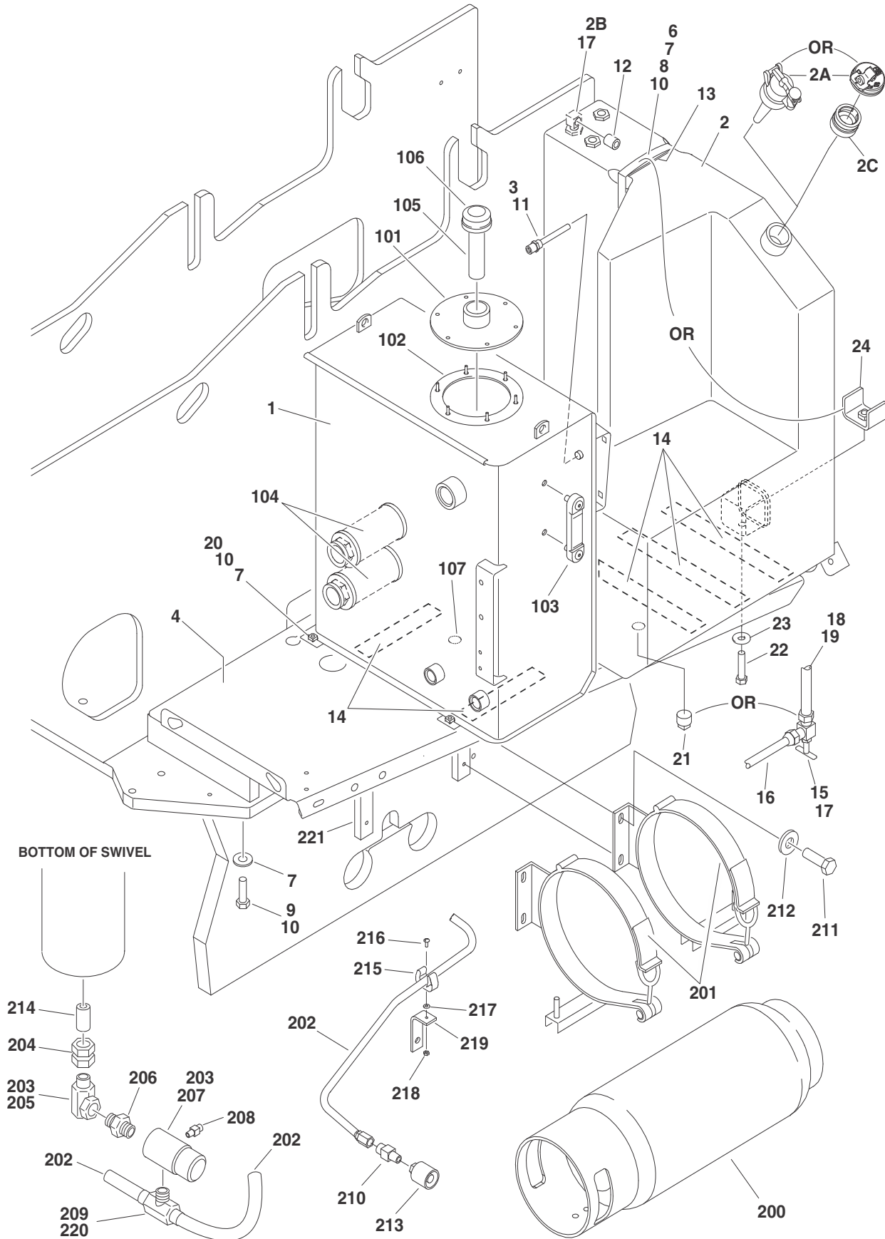
FIGURE 2-17. TANK INSTALLATIONS
