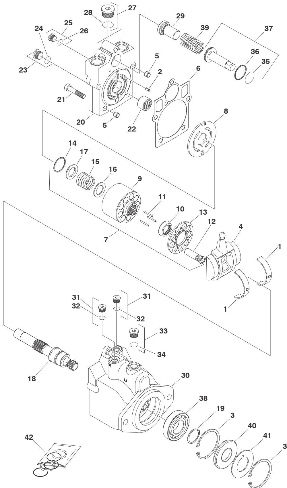
FIGURE 1-7. DRIVE MOTOR ASSEMBLY (USA BUILT MACHINES S/N 98766 TO S/N 0300177361 & CHINA BUILT MACHINES S/N B300000100 TO PRESENT) (SERVICE REPLACEMENT)
