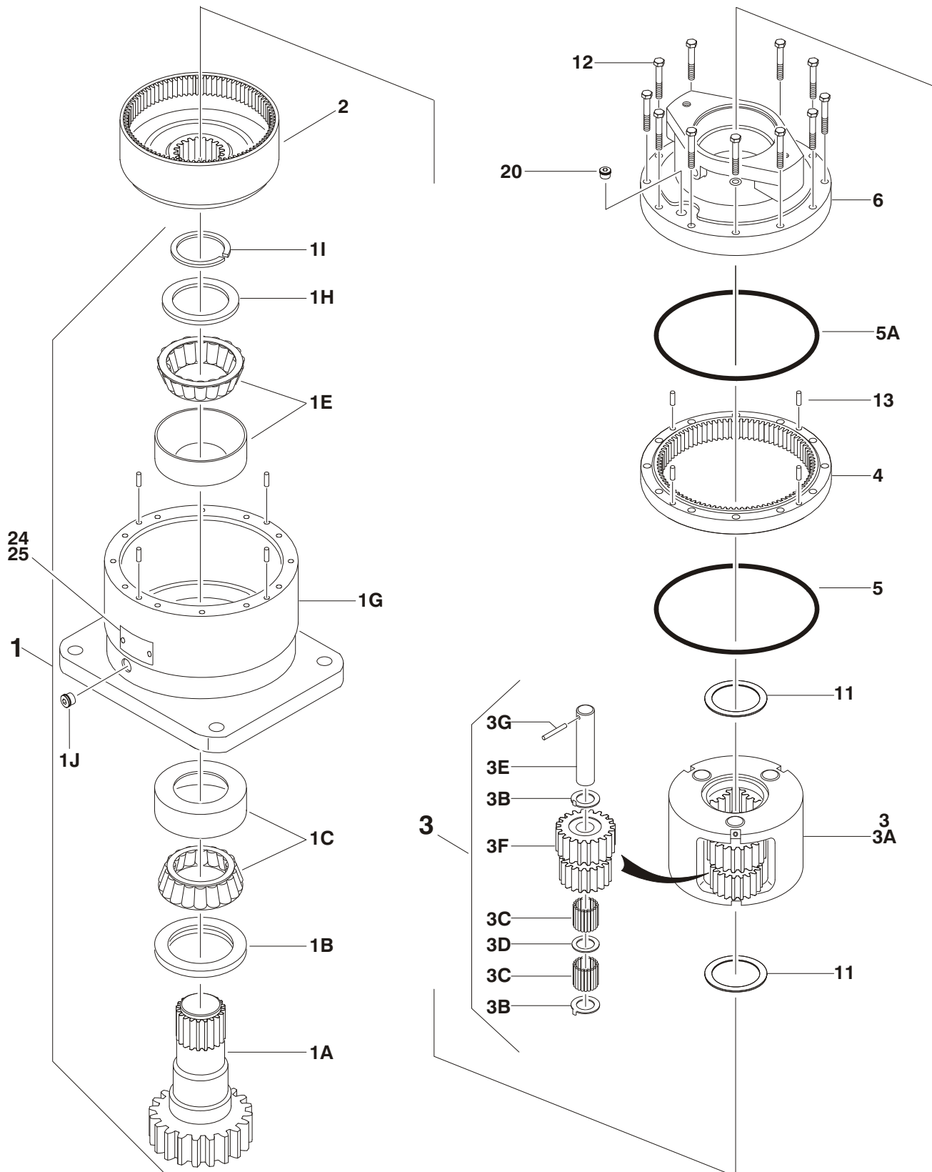
FIGURE 2-8.SWING MOTOR/BRAKE/HUB ASSEMBLY (PARKER/FAIRFIELD) (USA BUILT MACHINES S/N 0300137453 TO S/N 0300177361 & CHINA BUILT MACHINES S/N B300000100 TO PRESENT)
