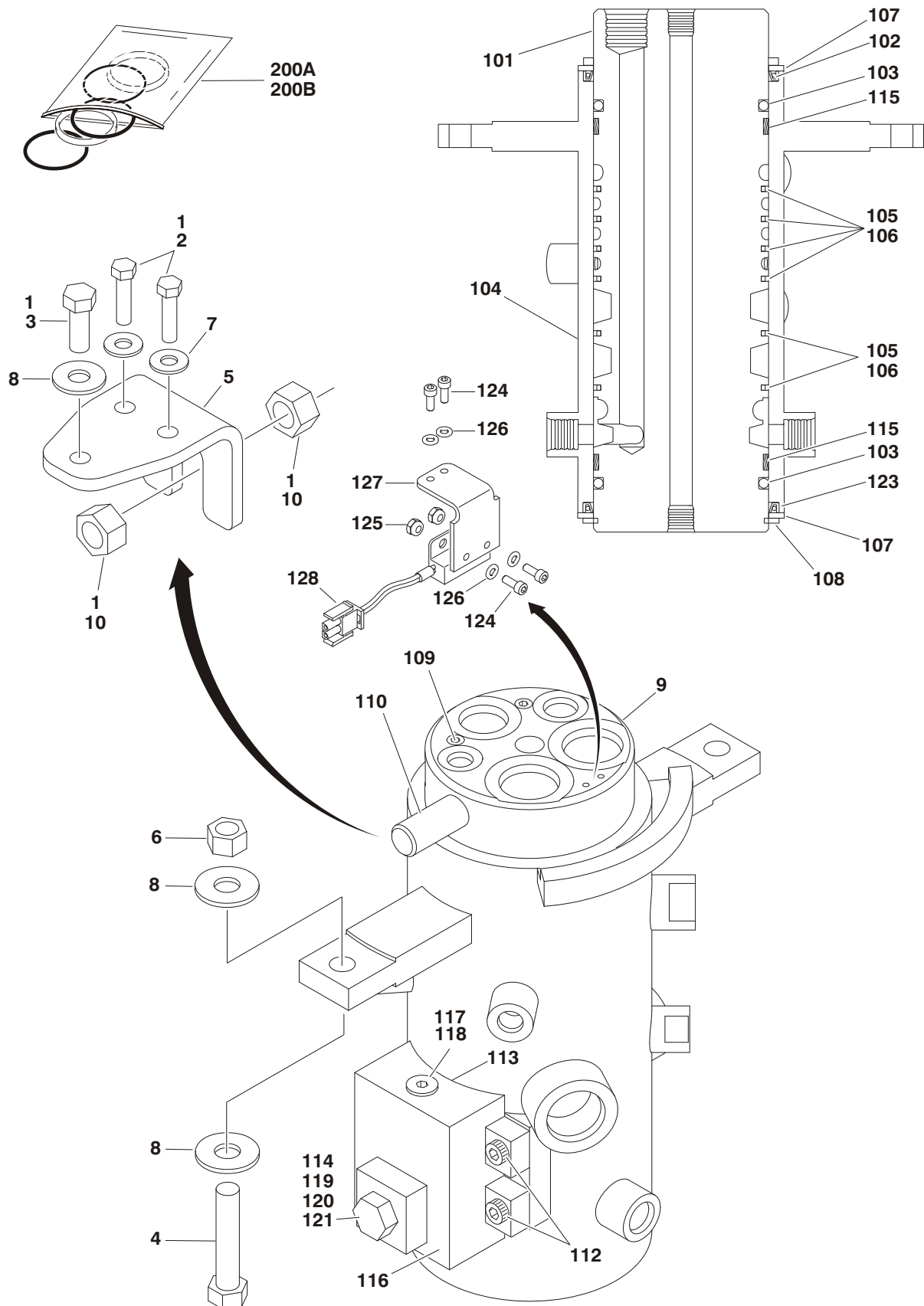
FIGURE 2-19. ROTARY COUPLING INSTALLATIONS (USA BUILT MACHINES S/N 0300138649 TO S/N 0300177361 & CHINA BUILT MACHINES S/N B300000100 TO PRESENT)
