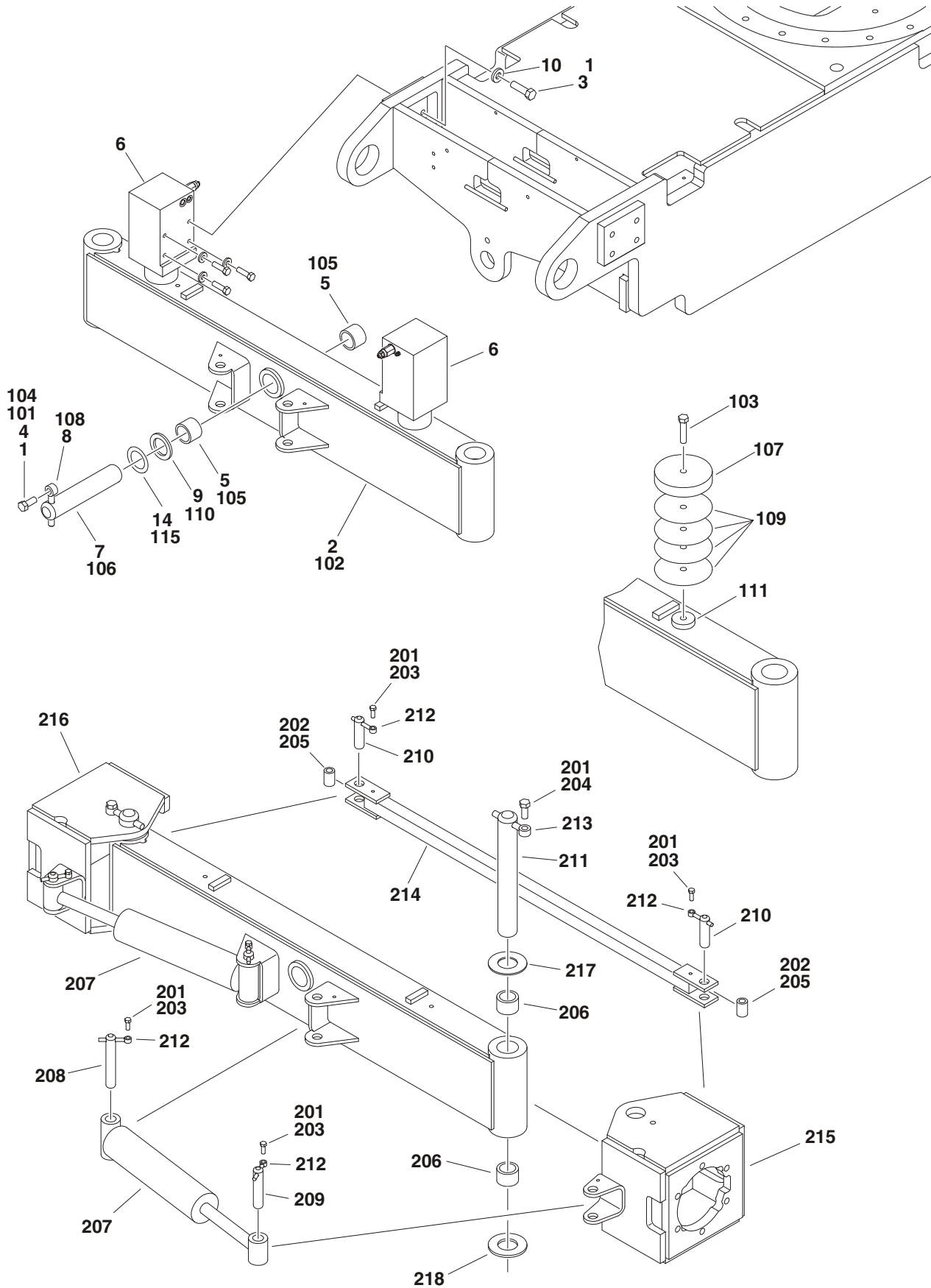
FIGURE 1-2. 4WD FRONT AXLE & STEERING INSTALLATIONS
