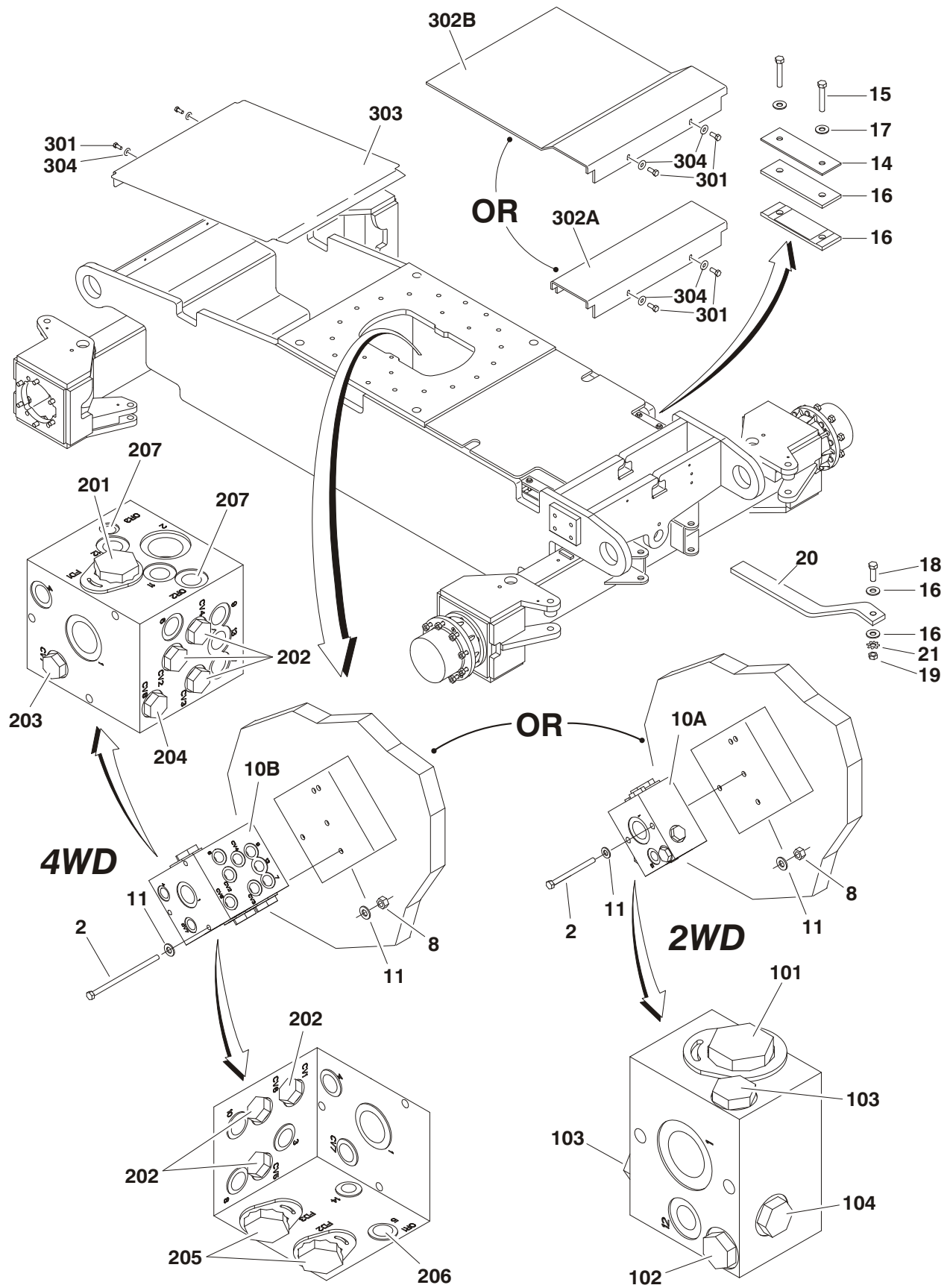
FIGURE 1-8. DRIVE VALVES & SHIELDS INSTALLATION (FRAME MOUNTED)
