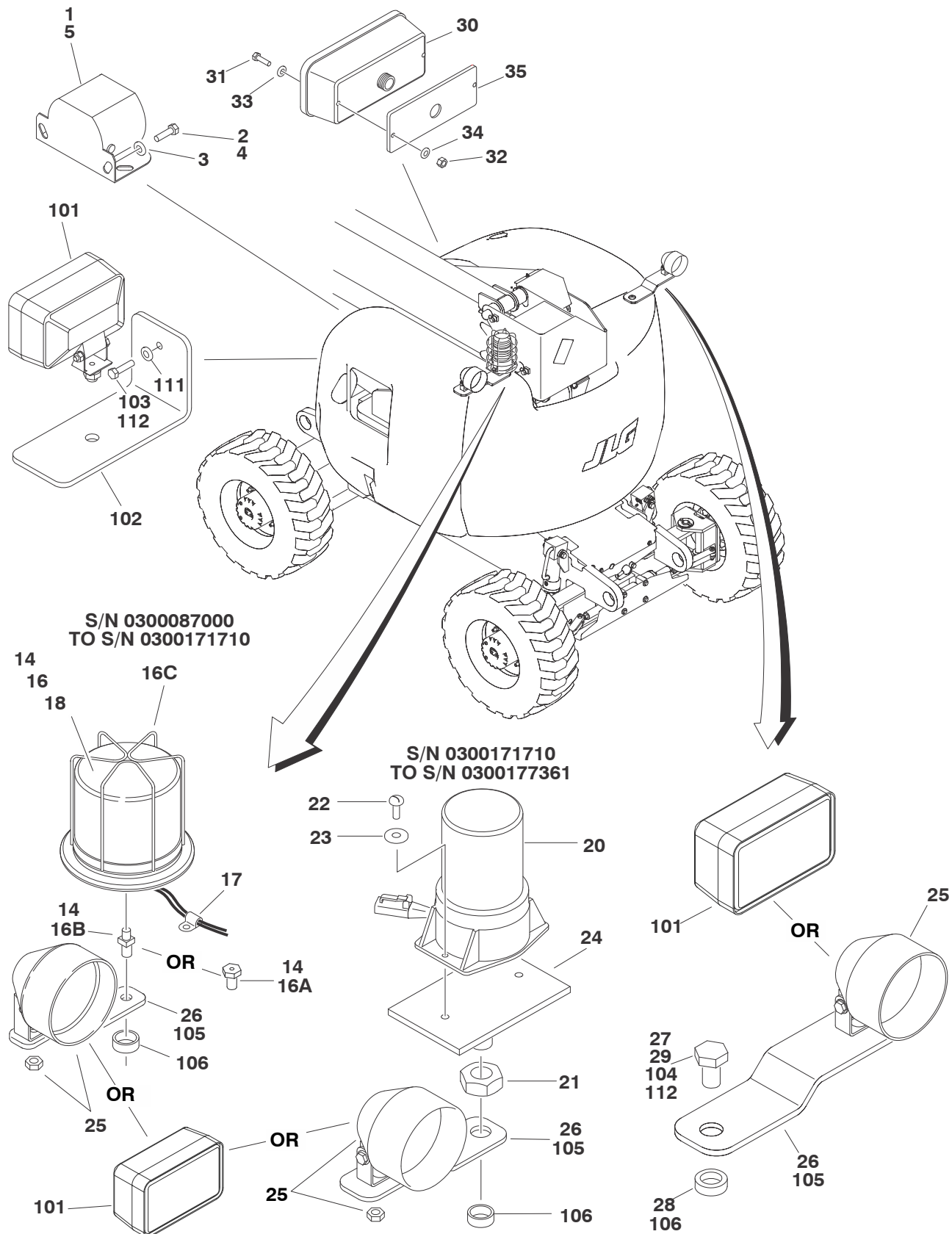
FIGURE 2-22. ELECTRICAL OPTIONS INSTALLATIONS (TURNTABLE MOUNTED)
