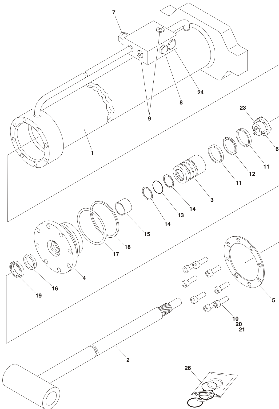
FIGURE 5-11. TELESCOPE CYLINDER ASSEMBLY - TOWER BOOM
