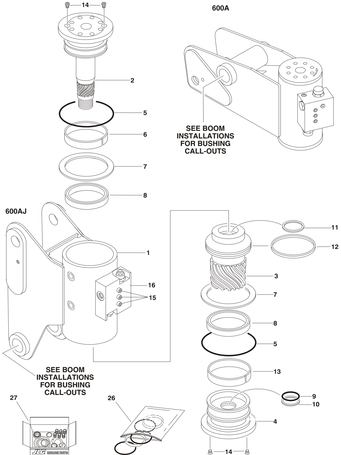
FIGURE 3-7. ROTATOR ASSEMBLIES
